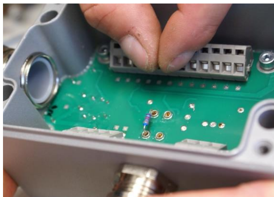
Figure 46: Insert resistor
